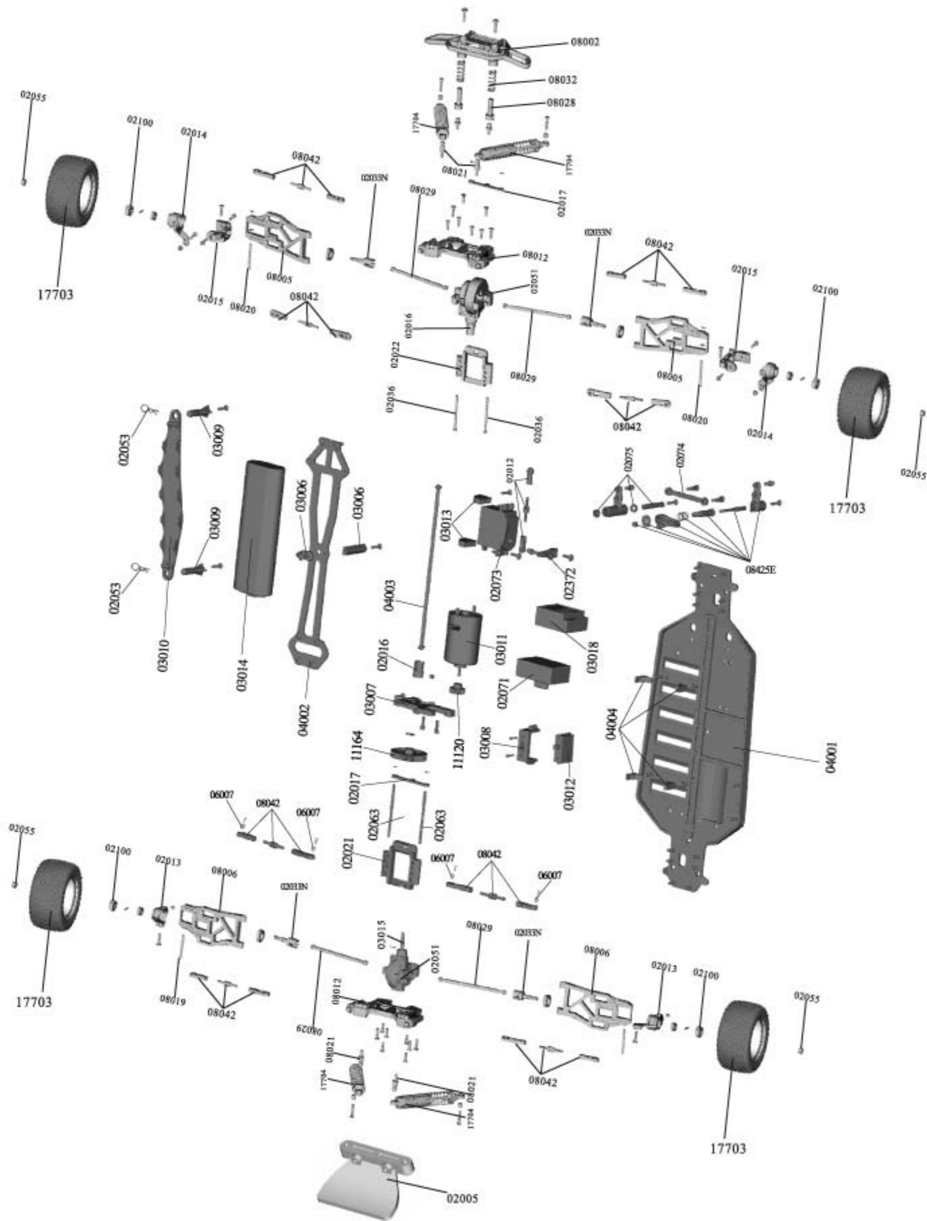
Full Assembly View
